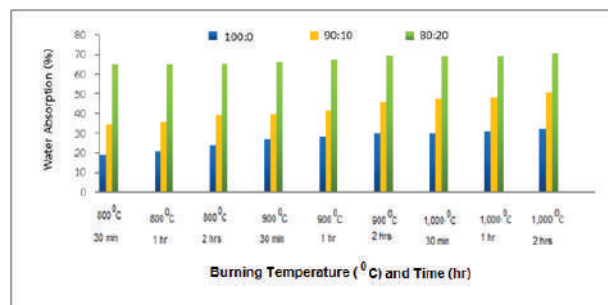
Figure 6 Water Absorption of Lightweight Expanded Clay Aggregate
