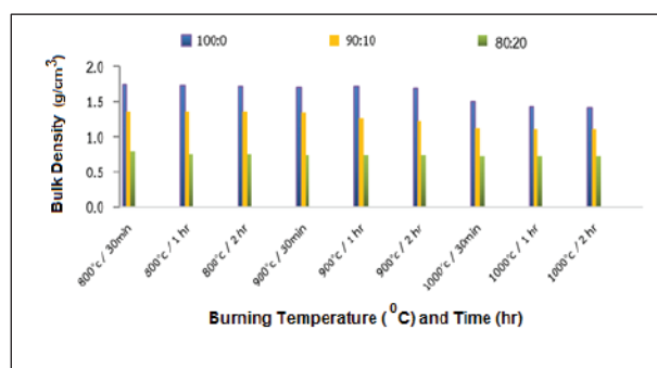
Figure 4 Bulk Density of Lightweight Expanded Clay Aggregate
