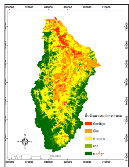
Figure 10 Map of suitable areas for flood evacuation
