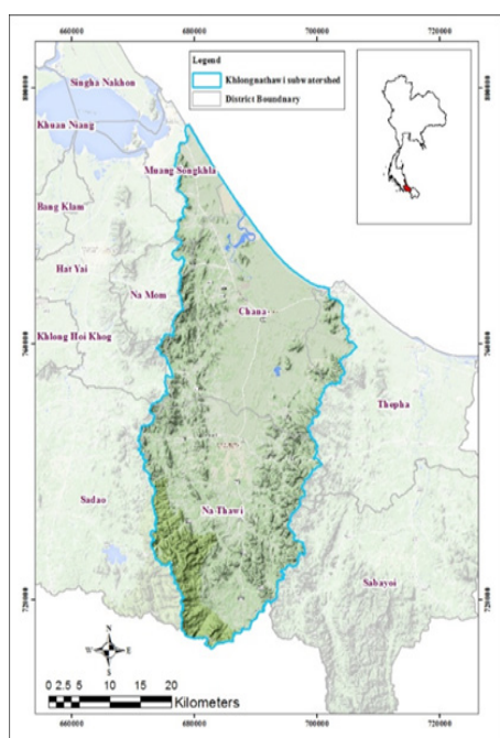
Figure 1 Location map of the study area (Khlung Nathawi subwatershed)
