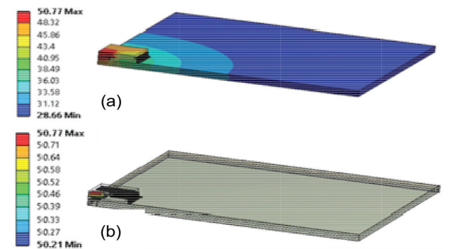
Figure 3 (a) Package and PCB temperature distribution of TQFP-EP no.1 and (b) Chip temperature distribution of TQFP-EP no.1
