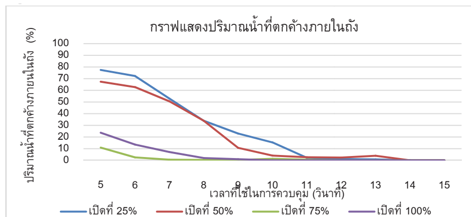
Figure 6 The percentage of the water pouring of remaining in the tank for the raw milk storage tank
