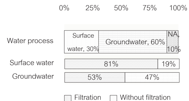
Figure 3 Water process in Sakon Nakhon Province
