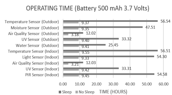
Figure 8 Operating time of each sensor node
