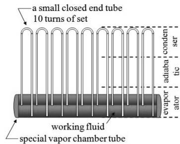
Figure 1 Shows the SCEHP/SVCs structure.
