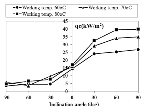
Figure 10 Heat flux with variations of inclination angle for various working temperature. (SCE: 2mm ID, SVC: 17.5mm ID, section length: 50mm, R-134a, filling ratio: 30%)
