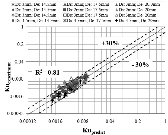
Figure 12 Comparison of experimental Ku vs. predicted Ku.
