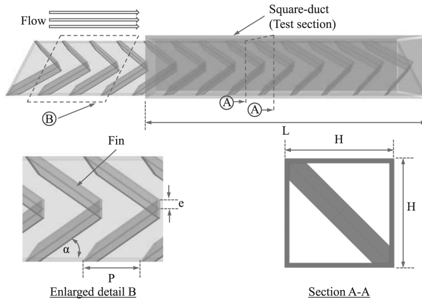
Figure 2 Test section with V-shaped fins
