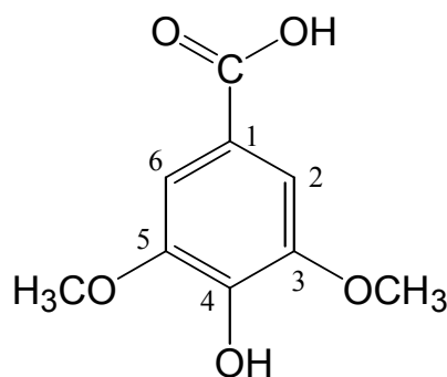
Figure 1 Chemical structure of the isolated compound (syringic acid)
