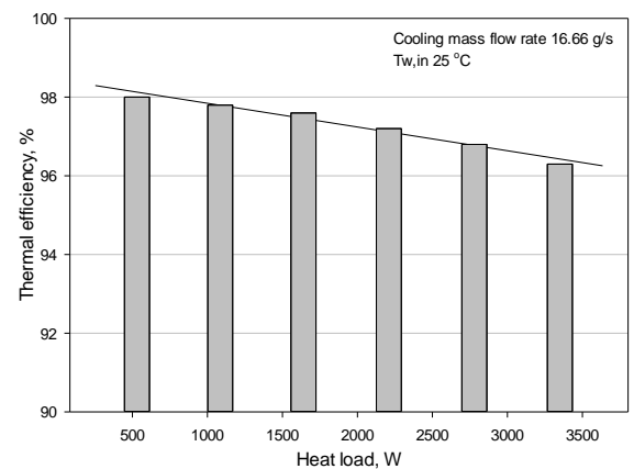
Figure 1 Thermal efficiency of experimental equipment
