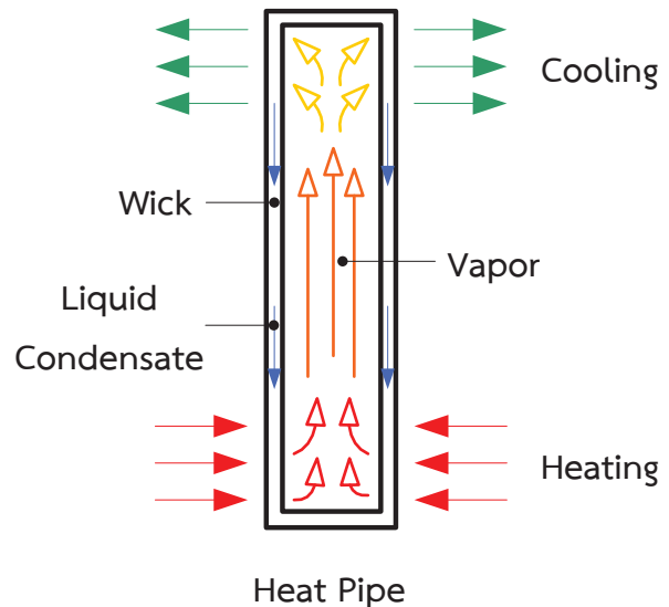
Figure 1 Heat Pipe
