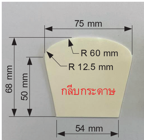
Figure 6 Dimensions of the paper petal
