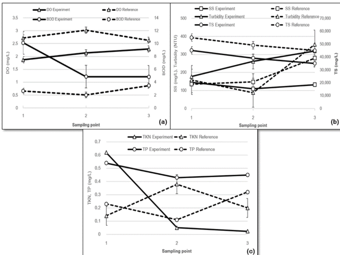
Figure 2 Water quality variation in Mangrove forest in front of The Royal LERD Project (Experiment) and Reference mangrove (Reference) from station 1, 2 and 3 (a) DO and BOD (b) Suspended solid (SS), Turbidity and Total Solid (TS) (c) TKN and Total Phosphorus (TP)
