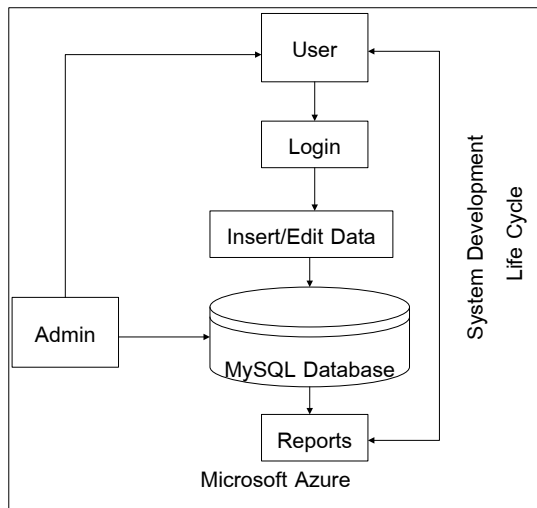
Figure 2 Database Design
